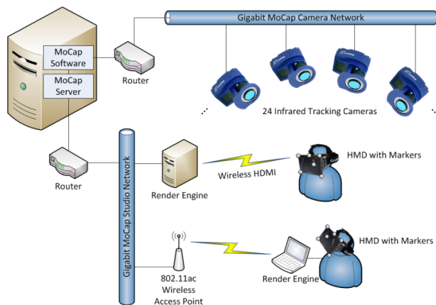
Figure 1. Block diagram of the Immersive VR Space.
